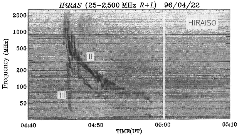
Fig. 6. Dynamical spectrum of April 22, 1996, event from Hiraïso Terrestrial Research Center: type III and type II bursts emitted in the corona (after [21])
