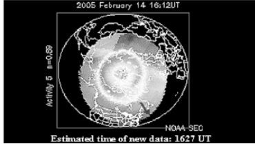
Fig. 8. Example of data delivered from Space Weather Centers
