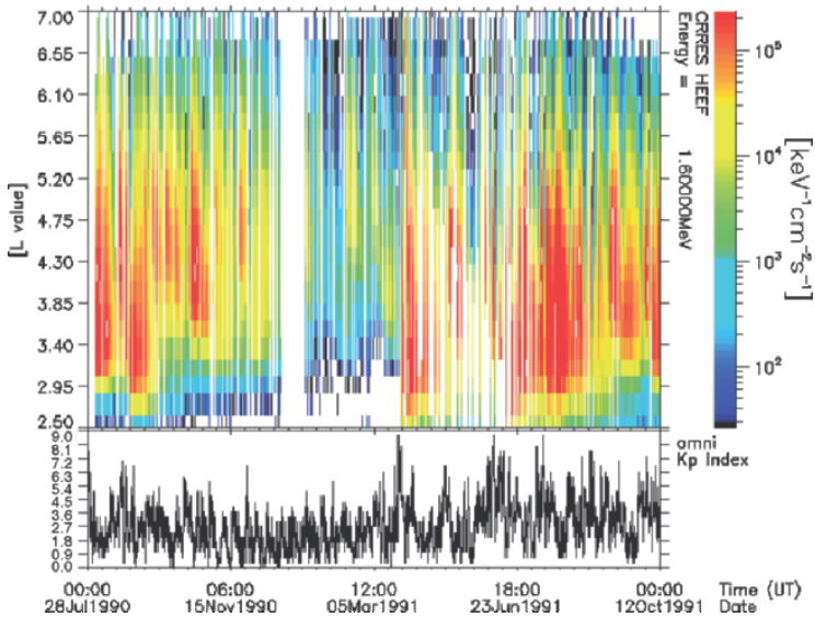
Fig. 22. Flux of 1.6 MeV electrons measured by the HEEF detector on CRRES for 14 months
