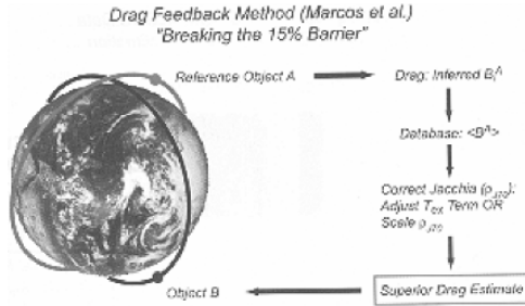
Fig. 30. Technological approach to estimate the thermospheric drag [56]
