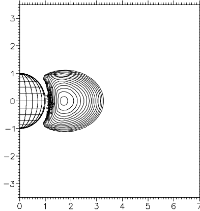
Fig. 11. Proton radiation belt
