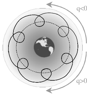
Fig. 9. Drift movement for an equatorial charged particle (which does not bounce \alpha_{eq} = 90^\circ )
